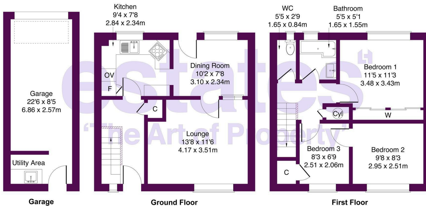
Ground Floor Not to Scale. Produced by The Plan Portal 2026 For Illustrative Purposes Only.
